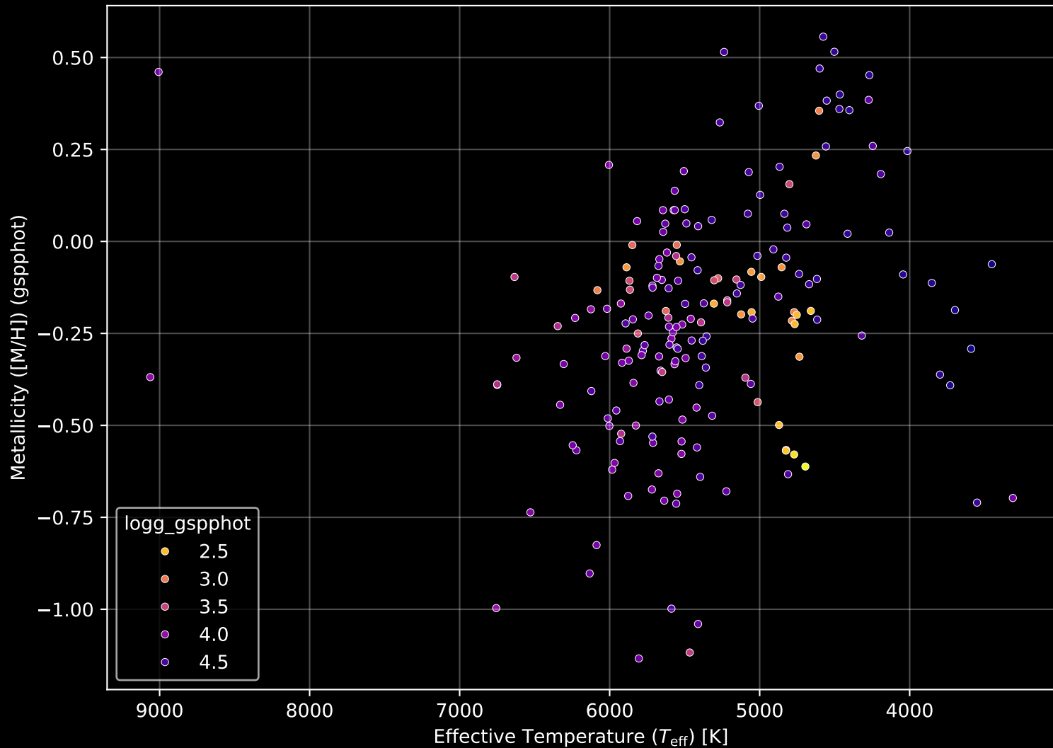
APOGEE DR17 Field: [091-59_MGA] Stellar Population Parameters (n= 195)
