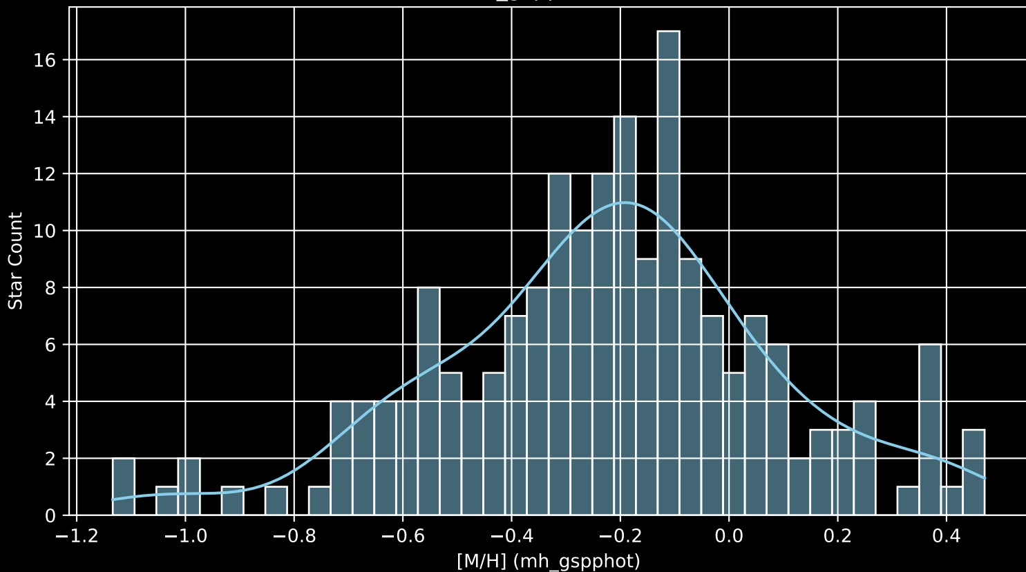
APOGEE DR17 Field: [091-59_MGA [M/H] (mh_gspphot) (n= 192)
