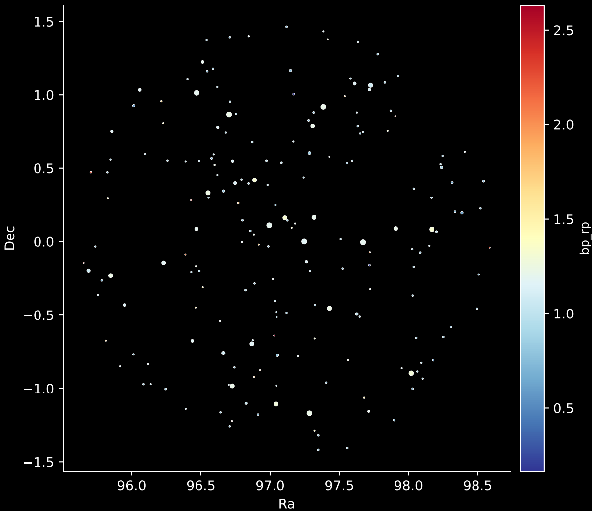
APOGEE DR17 Field: [091-59_MGA] Stars: 195
