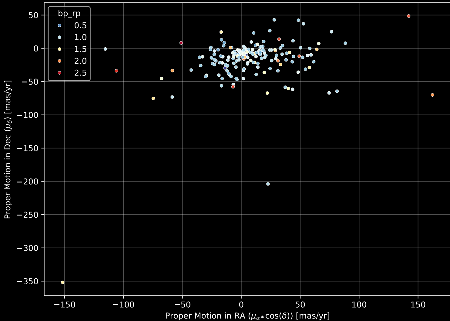
APOGEE DR17 Field: [091-59_MGA] Proper Motion Diagram (n= 195)
