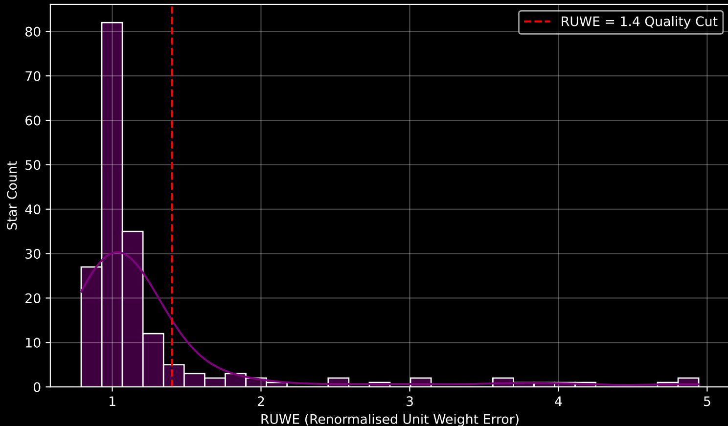
GAPOGEE DR17 Field [091-59_MGA] RUWE Distribution (n= 186)
