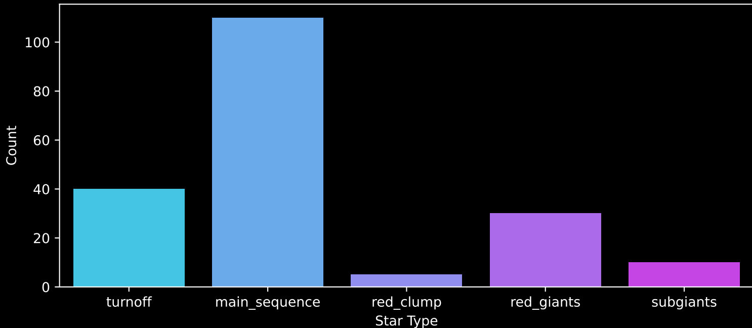
APOGEE DR17 Field: [091-59_MGA] Count plot of Star Type
