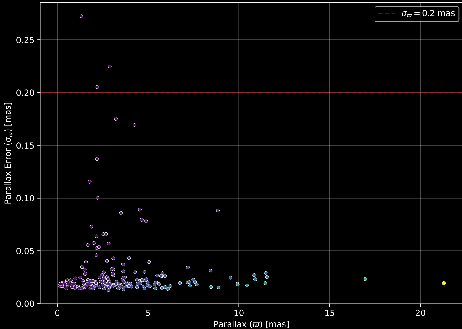
APOGEE DR17 Field: [091-59_MGA] Parallax Quality (n= 195)
